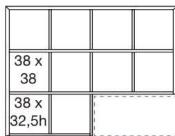
KEOPE Art. 590 libreria Dx o Sx bookcase Right / Left cm. 168 x 31 x 126 h
